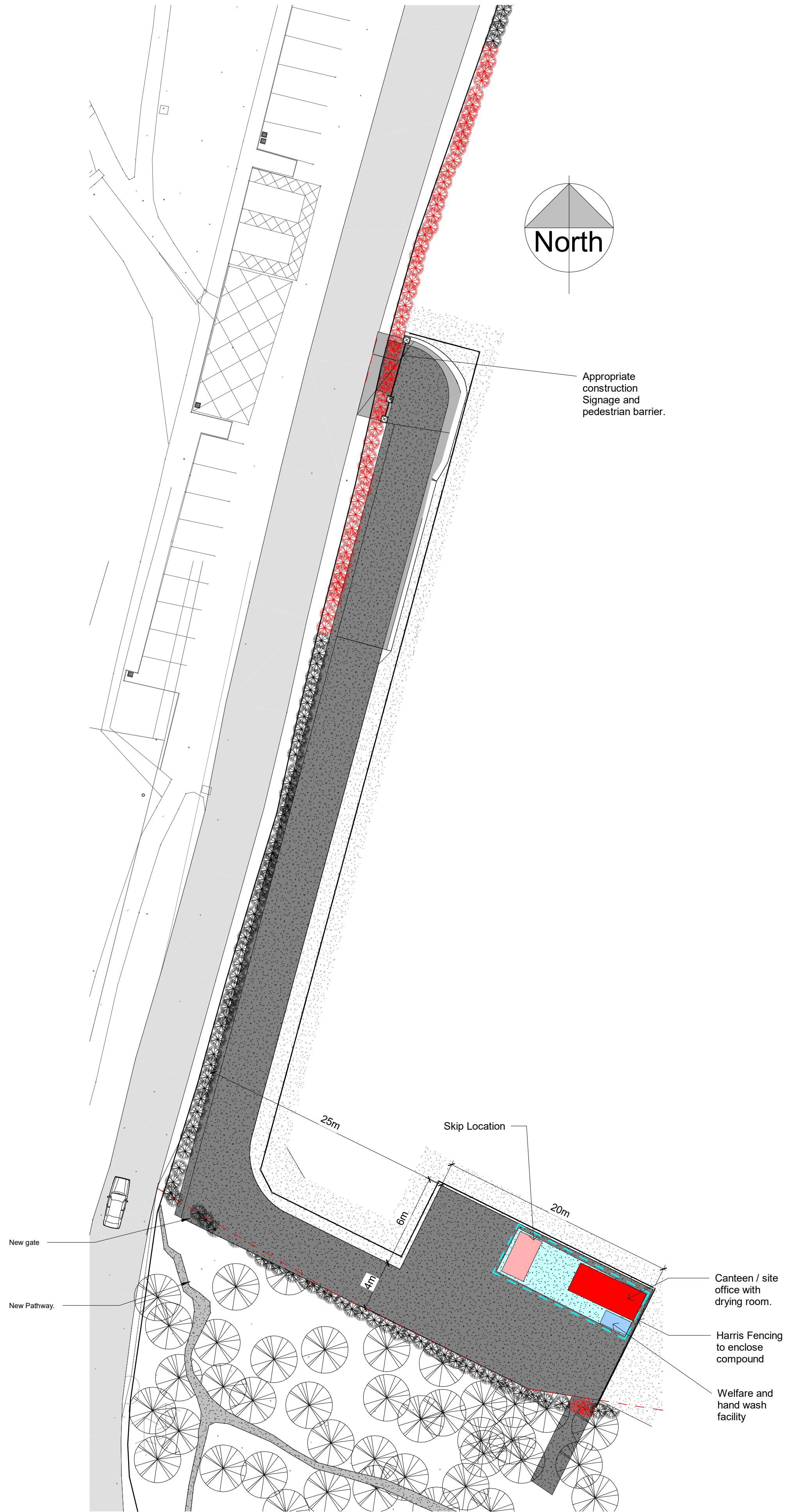
Site Compound Phase 2 1 : 250
