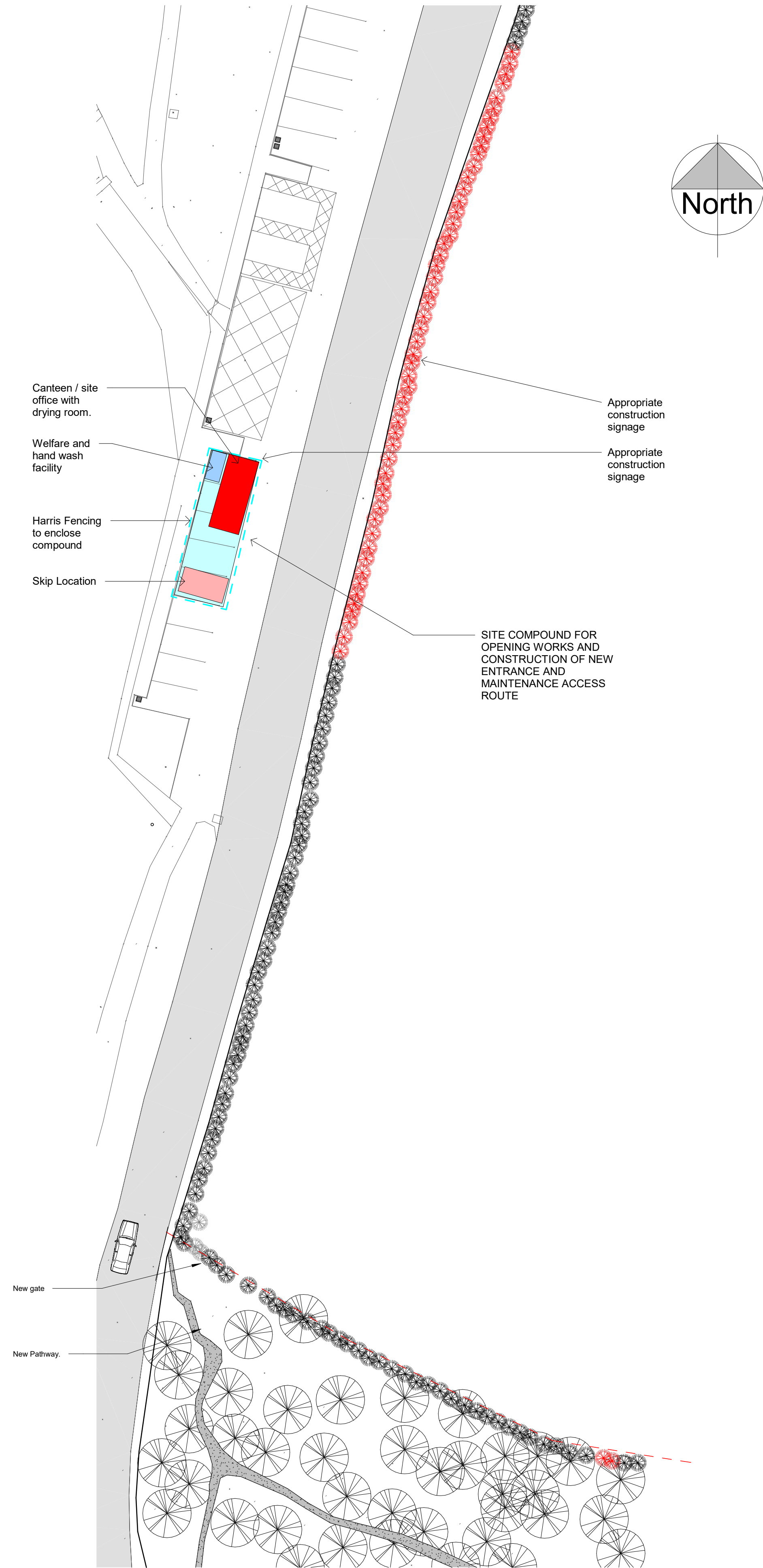
Site Compound Phase 1 1 : 250
